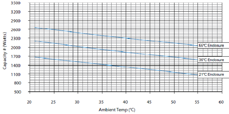
VA082025GXXXS Capacity Curves 230V/50Hz
