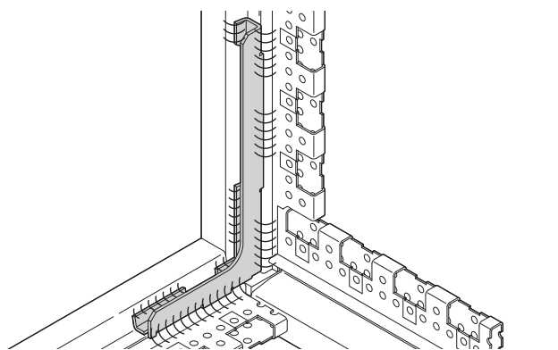
Welded basic frame with strengthening brackets
