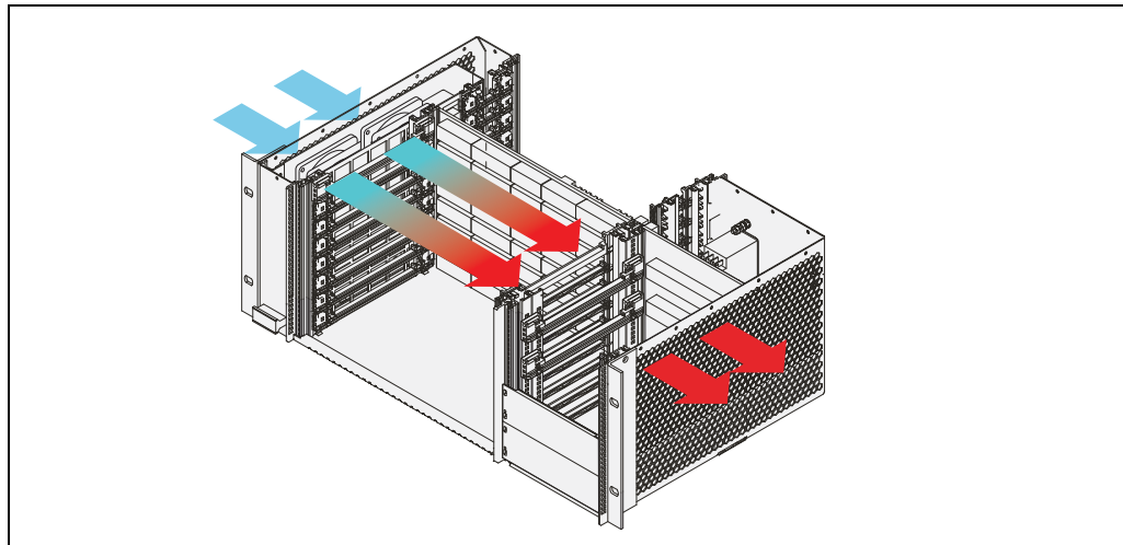
Figure 5: Airflow
