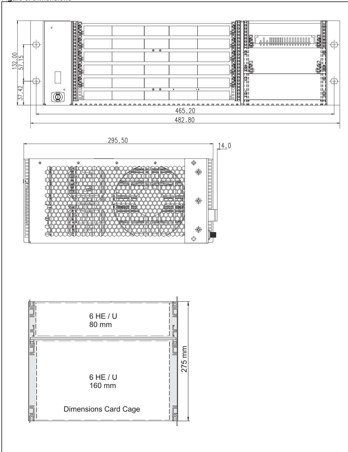
Figure 6: Dimensions
