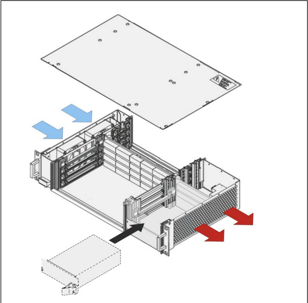
Figure 5: Air Flow
