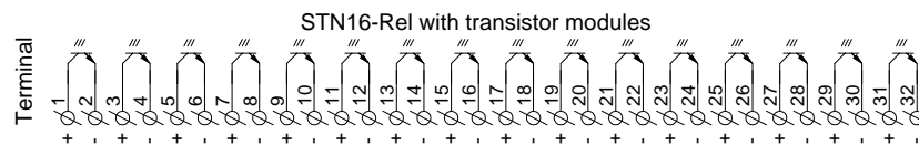
Screw terminal
