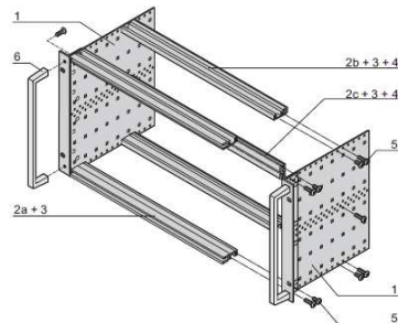
Without front handle 06102007 With front handle 0611003
