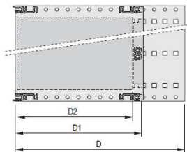
D = overall depth, D1 = insertion depth, D2 = board depth 0610052
