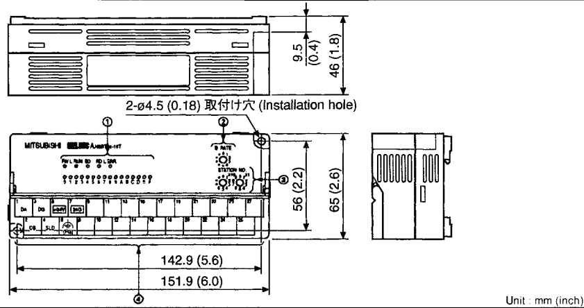
Unit: mm (inch)
